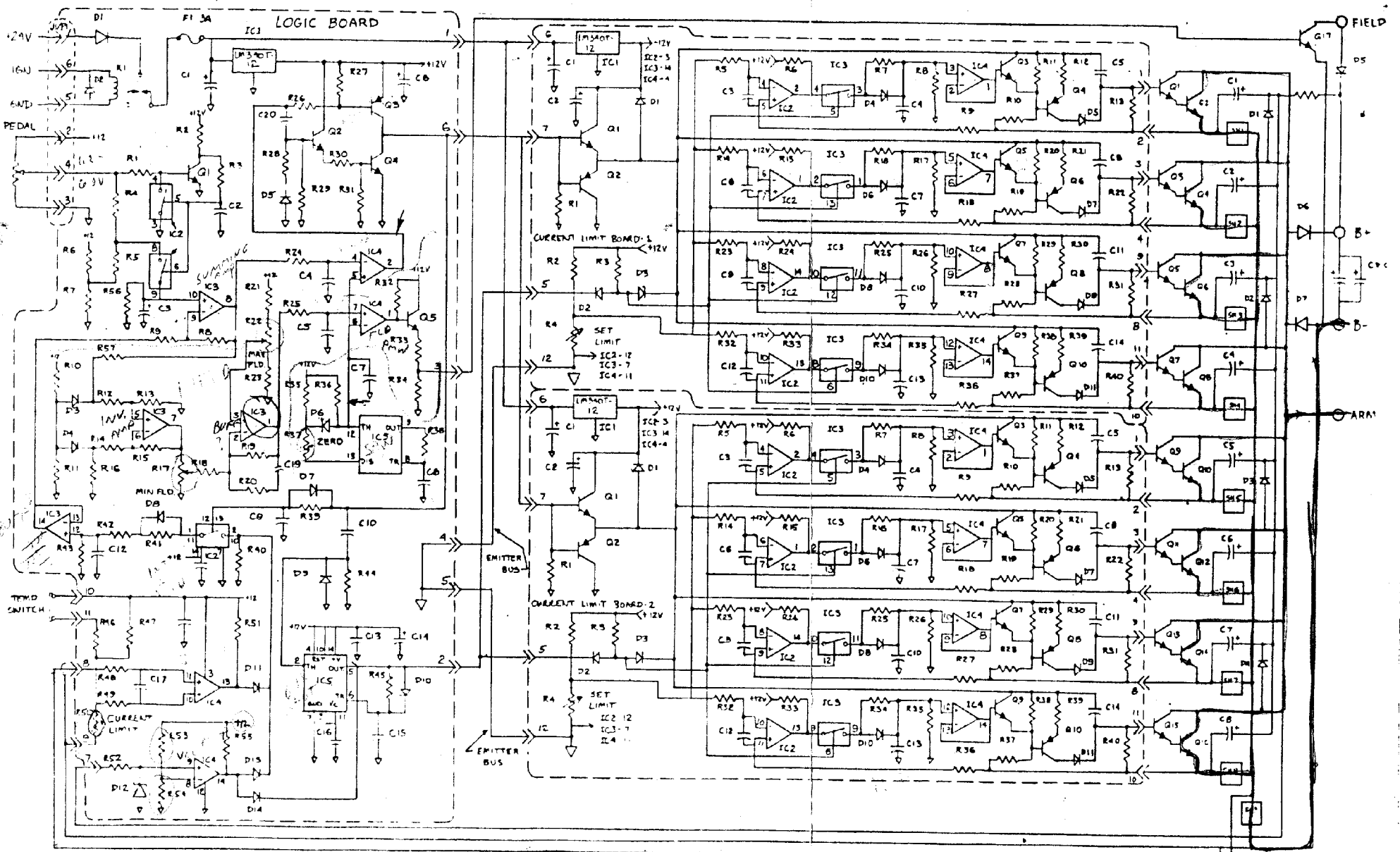
FIGURE 23. PMC CONTROLLER SCHEMATIC
