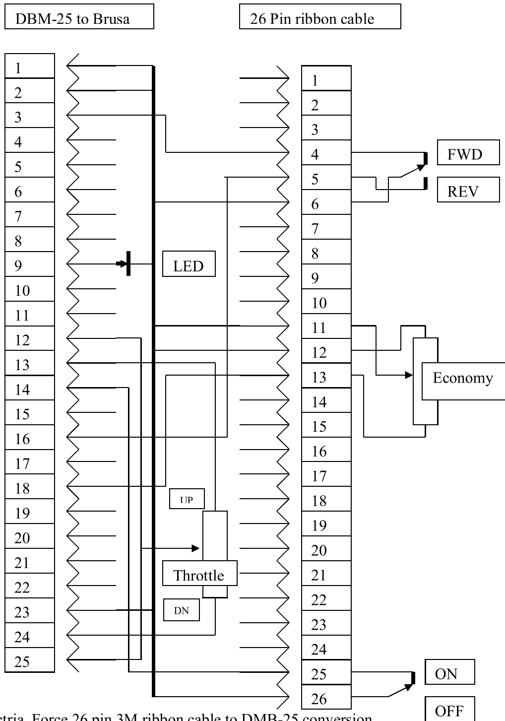
Solectria Force 26 pin 3M ribbon cable to DMB-25 conversion
